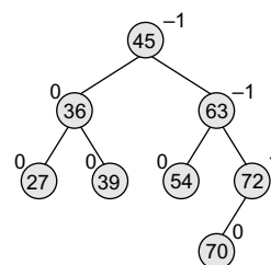
Figure 10.38 AVL tree
