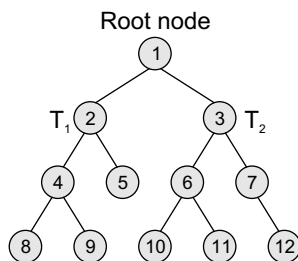
Figure 9.3 Binary tree
