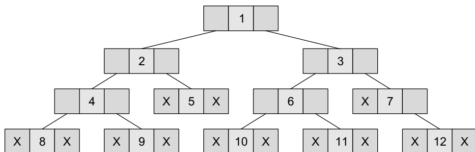
Figure 9.9 Linked representation of a binary tree
